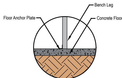
Floor Anchor Option
