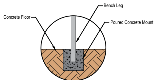
Post Mount Option
